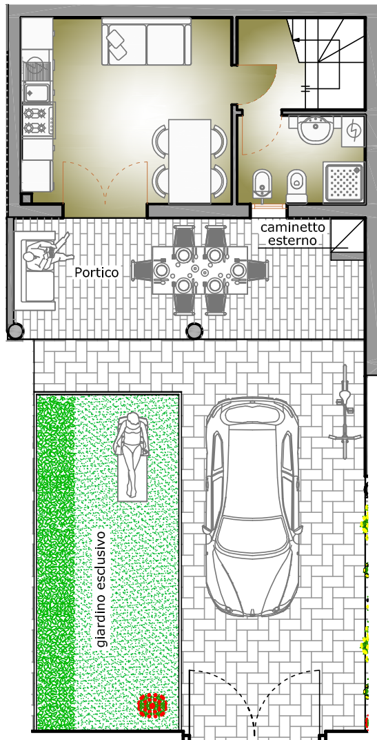
PIANO TERRA
